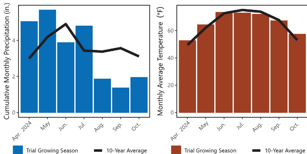
FIGURE A2. Modelled mean monthly temperature and rainfall at each trial site during the study period and the ten-year historic averages. Data is from the NasaPOWER climate dataset. [5, 6]
